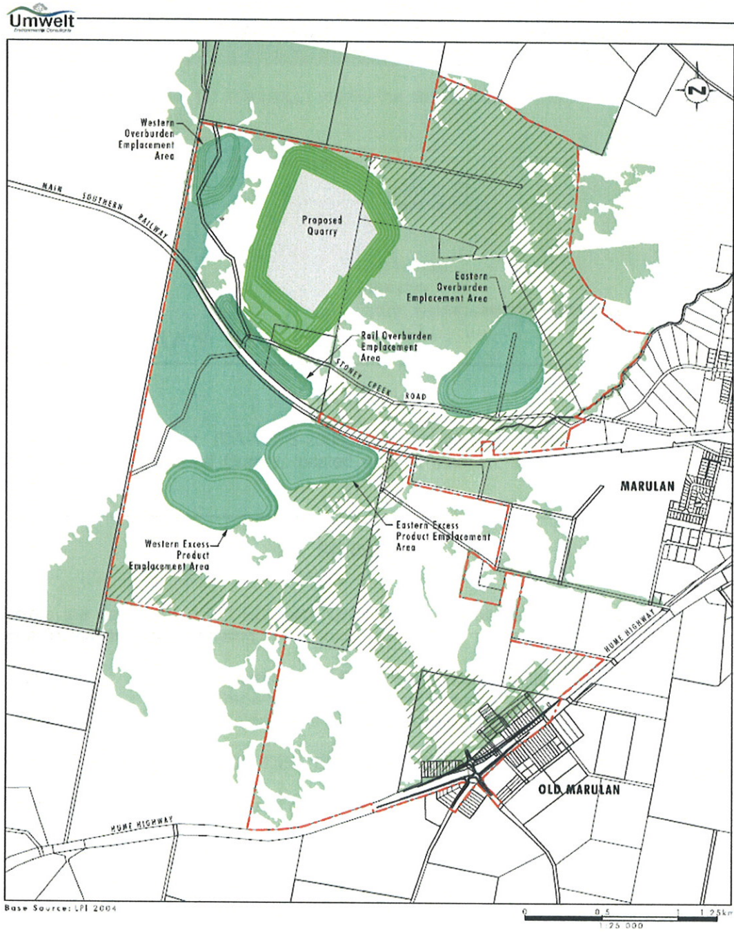
FIGURE 4.7 Year 30 Conceptual Final Rehabilitation
