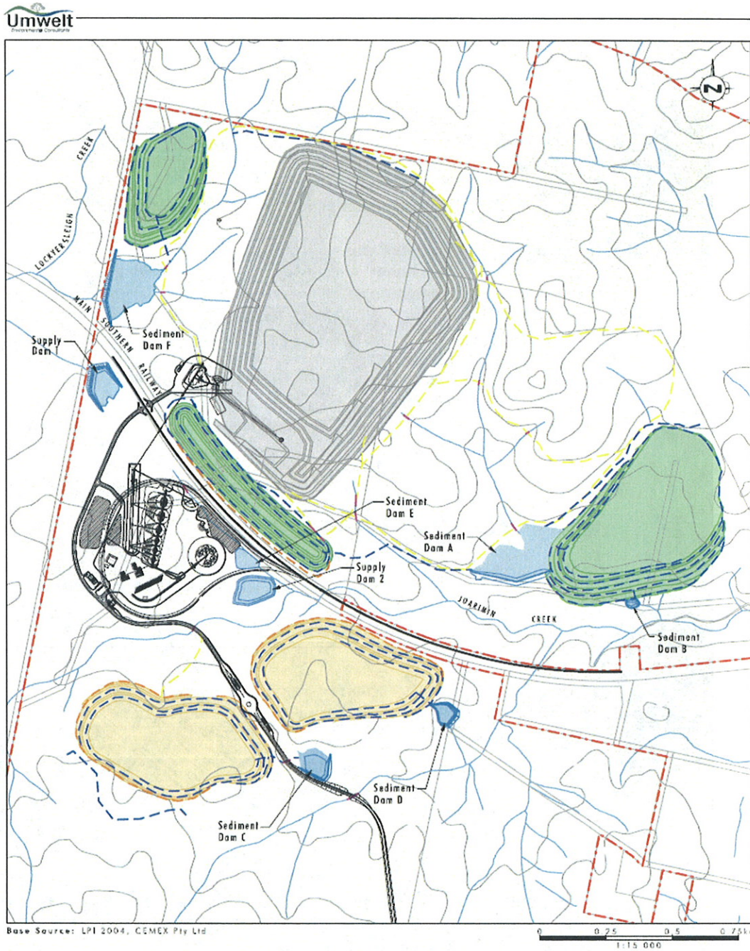
FIGURE 4.1 Proposed Water Management Controls - Year 30
